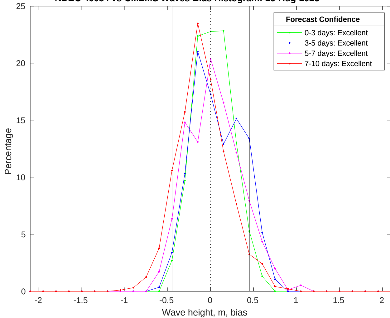
NDBC 46054 vs CMEMS Waves Bias Histogram: 16-Aug-2025
