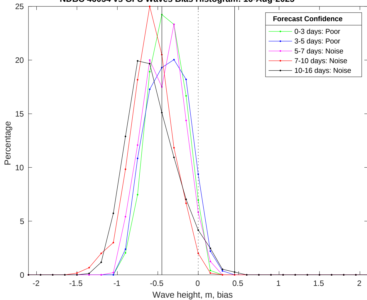
NDBC 46054 vs GFS Waves Bias Histogram: 16-Aug-2025
