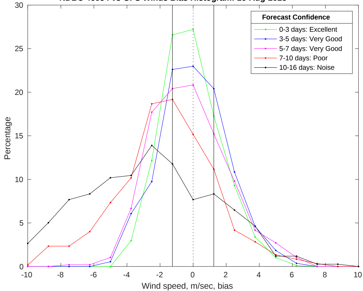
NDBC 46054 vs GFS Winds Bias Histogram: 16-Aug-2025
