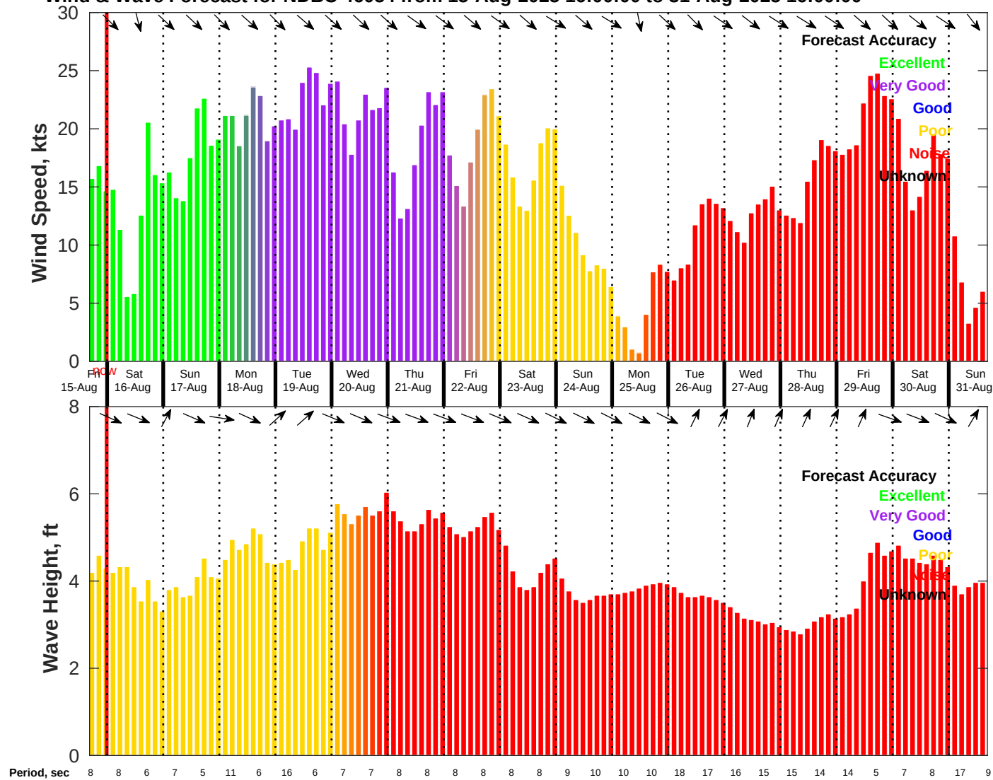
Wind & Wave Forecast for NDBC 46054 from 15-Aug-2025 16:00:00 to 31-Aug-2025 16:00:00
