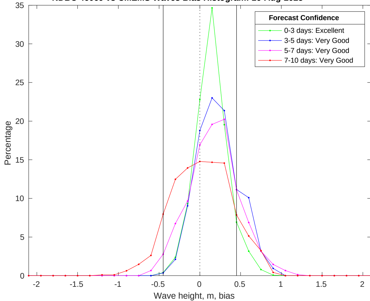
NDBC 46069 vs CMEMS Waves Bias Histogram: 16-Aug-2025
