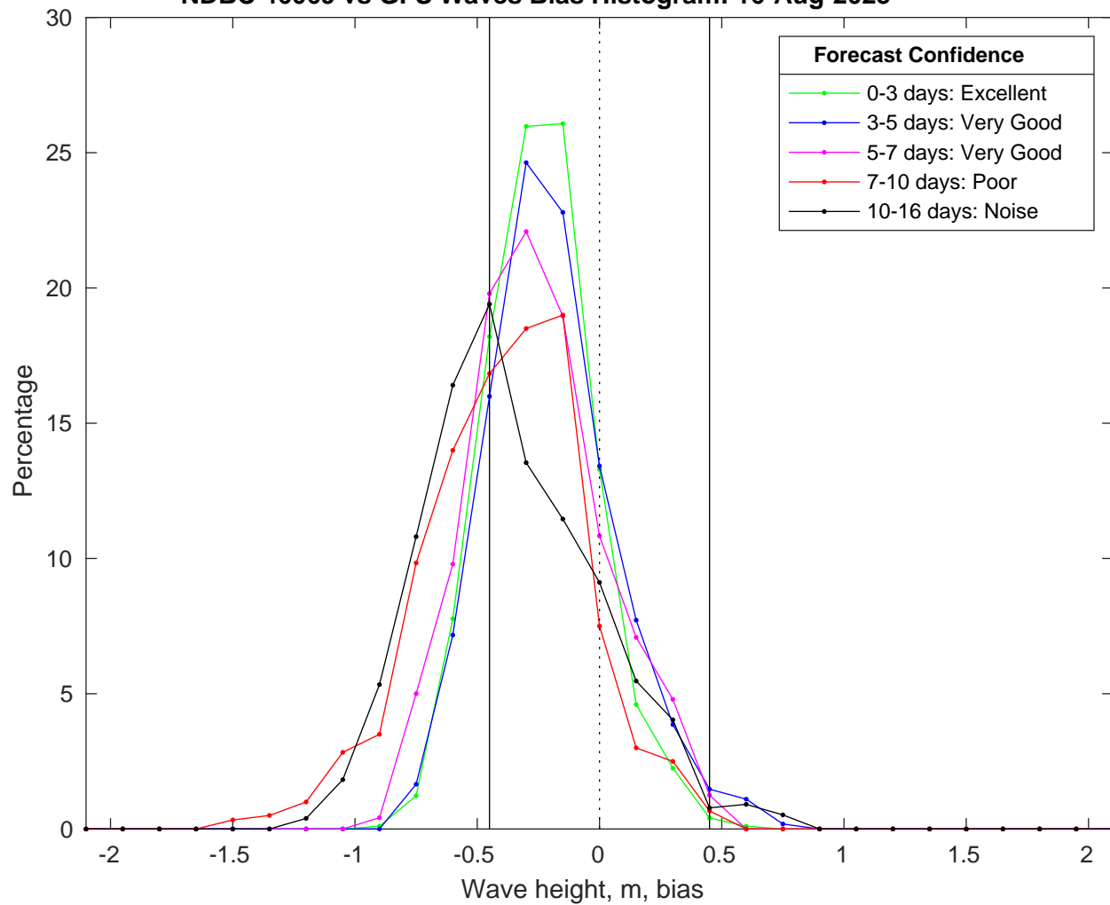
NDBC 46069 vs GFS Waves Bias Histogram: 16-Aug-2025
