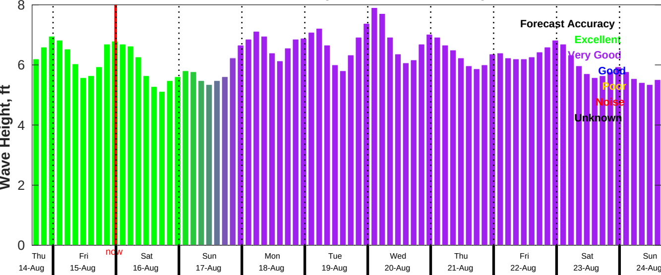
CMEMS Wave Forecast for NDBC 46069 from 14-Aug-2025 16:00:00 to 24-Aug-2025 16:00:00
