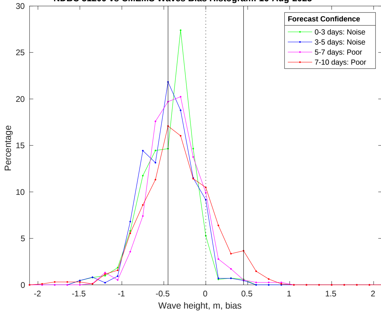
NDBC 51209 vs CMEMS Waves Bias Histogram: 16-Aug-2025
