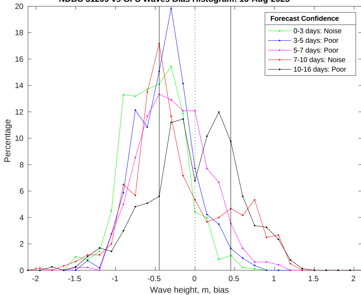
NDBC 51209 vs GFS Waves Bias Histogram: 16-Aug-2025
