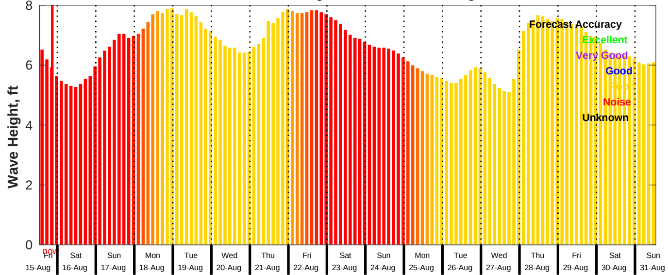
GFS Wave Forecast for NDBC 51209 from 15-Aug-2025 13:00:00 to 31-Aug-2025 13:00:00
