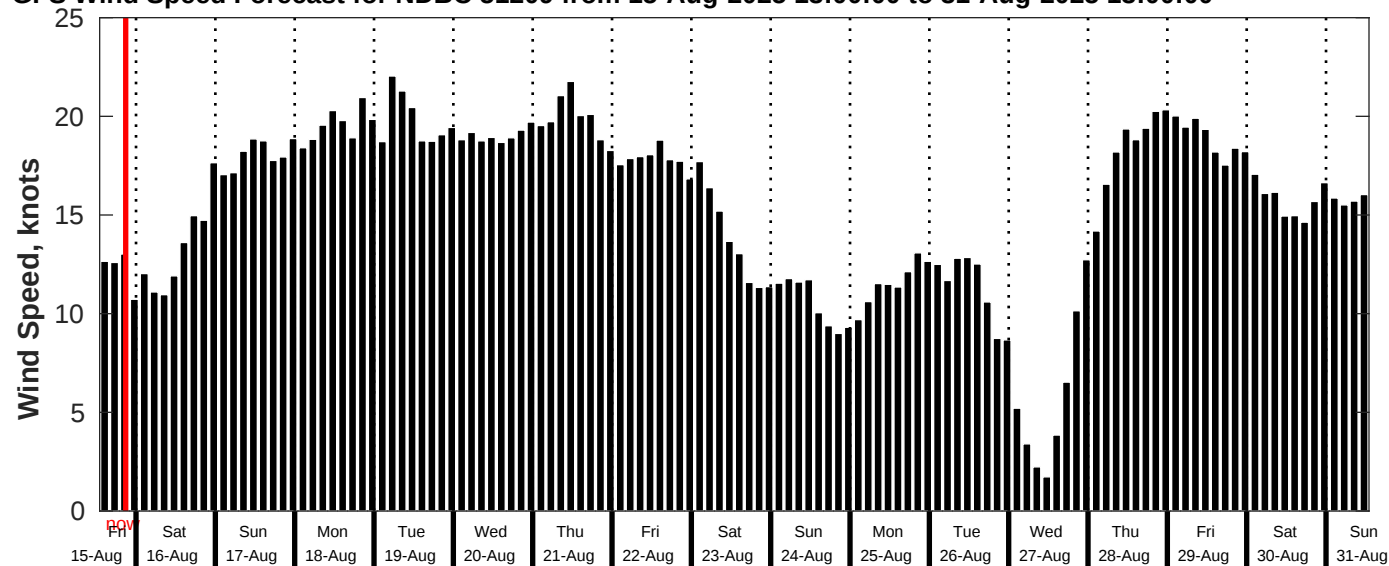
GFS Wind Speed Forecast for NDBC 51209 from 15-Aug-2025 13:00:00 to 31-Aug-2025 13:00:00
