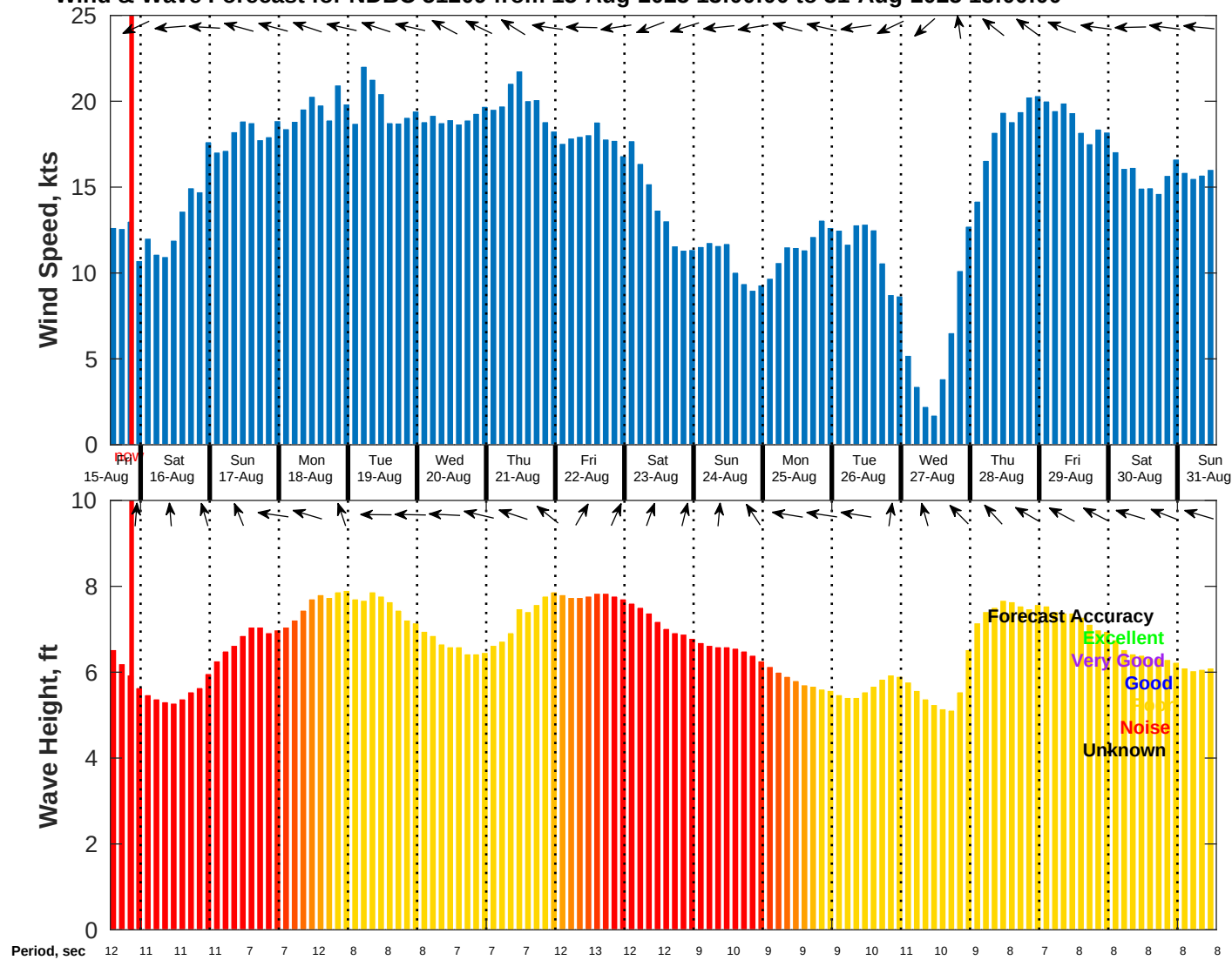
Wind & Wave Forecast for NDBC 51209 from 15-Aug-2025 13:00:00 to 31-Aug-2025 13:00:00
