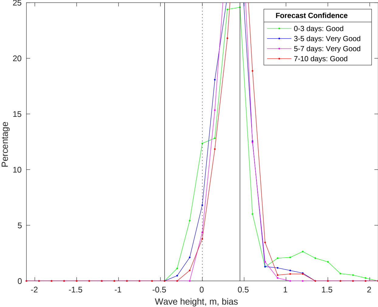
NDBC 51211 vs CMEMS Waves Bias Histogram: 16-Aug-2025
