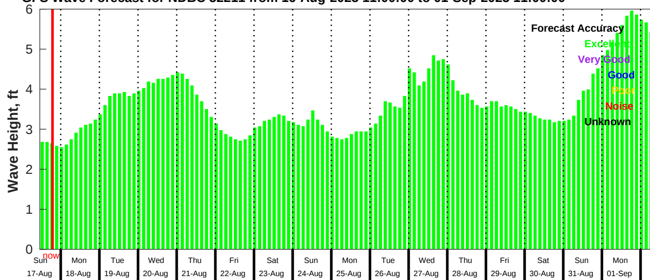
GFS Wave Forecast for NDBC 52211 from 16-Aug-2025 11:00:00 to 01-Sep-2025 11:00:00
