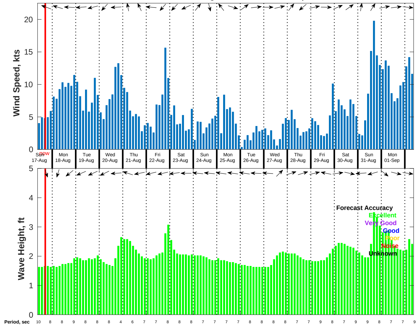
Wind & Wave Forecast for NDBC 52212 from 16-Aug-2025 09:00:00 to 01-Sep-2025 09:00:00
