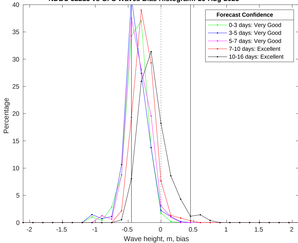
NDBC 52213 vs GFS Waves Bias Histogram: 16-Aug-2025
