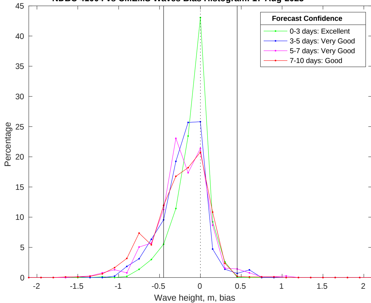
NDBC 41004 vs CMEMS Waves Bias Histogram: 17-Aug-2025
