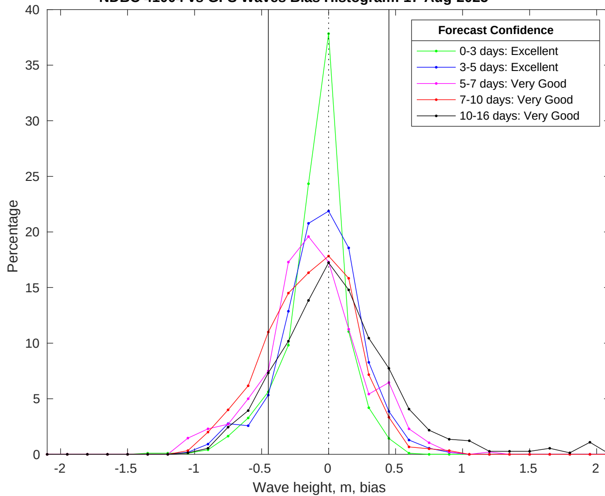
NDBC 41004 vs GFS Waves Bias Histogram: 17-Aug-2025
