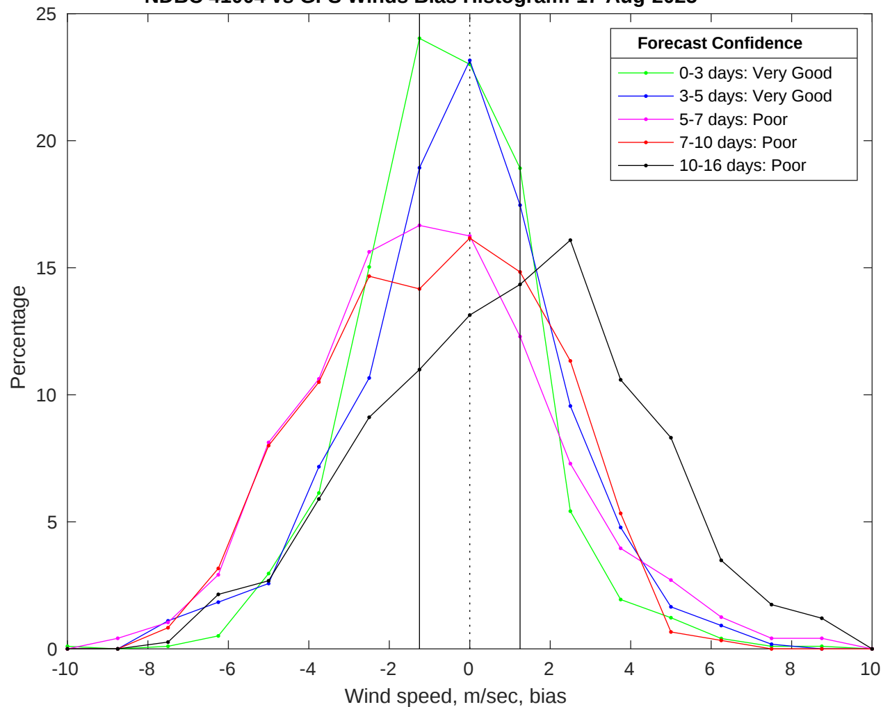
NDBC 41004 vs GFS Winds Bias Histogram: 17-Aug-2025
