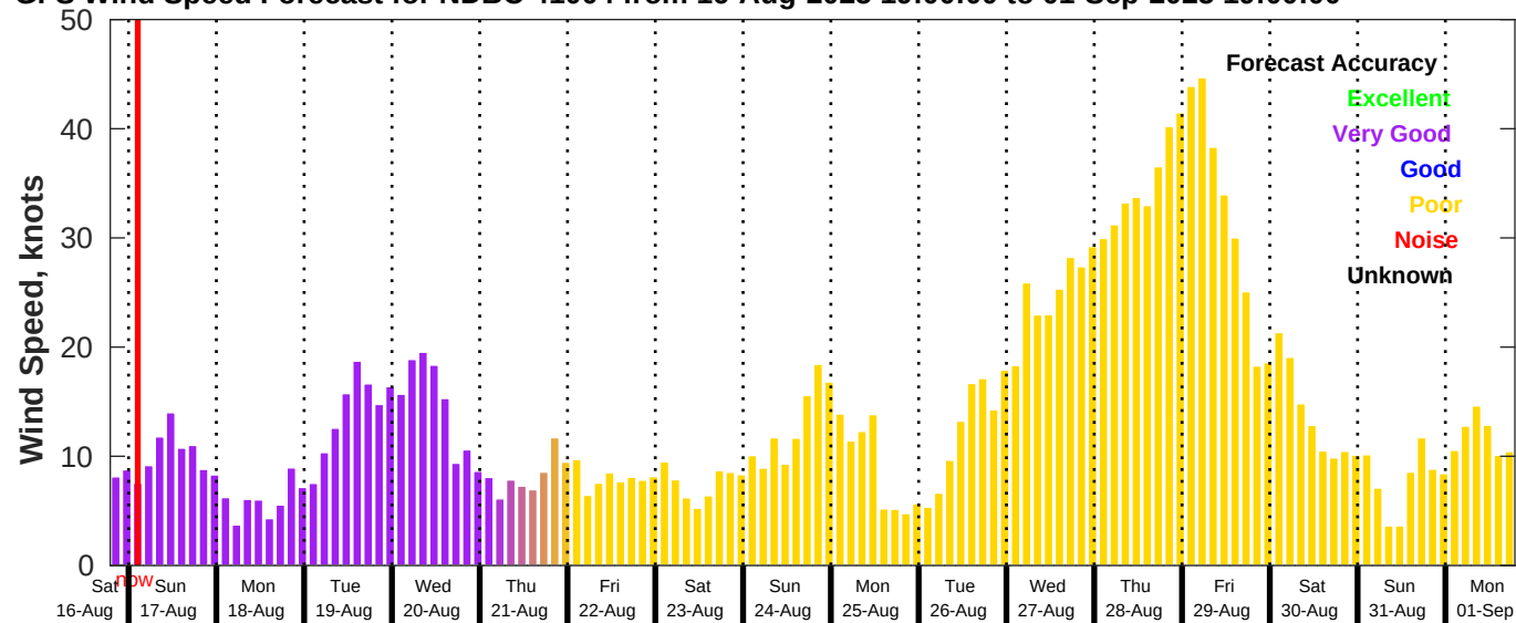
GFS Wind Speed Forecast for NDBC 41004 from 16-Aug-2025 19:00:00 to 01-Sep-2025 19:00:00
