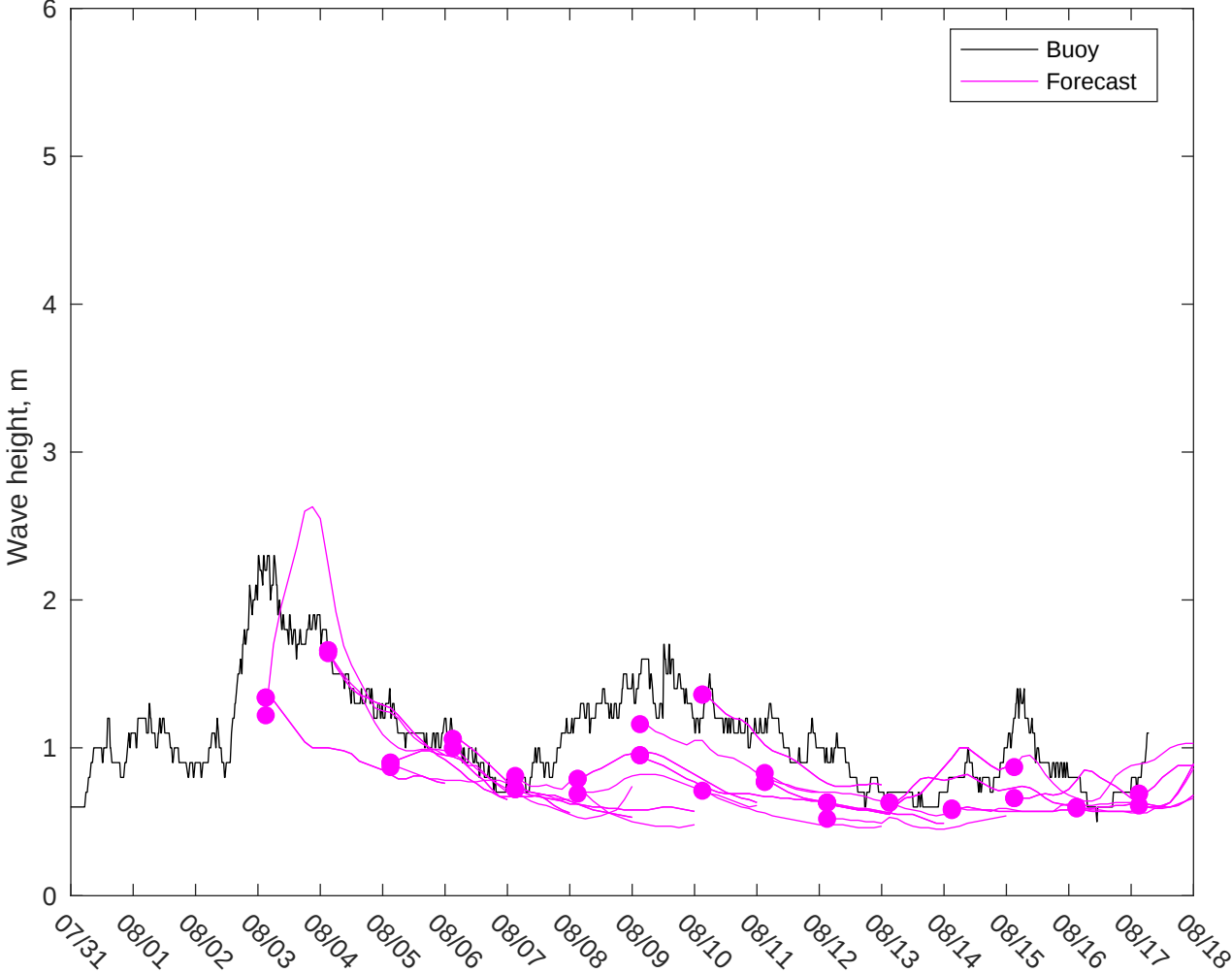
NDBC 41013 vs CMEMS Waves: 7 to 10 day forecast
