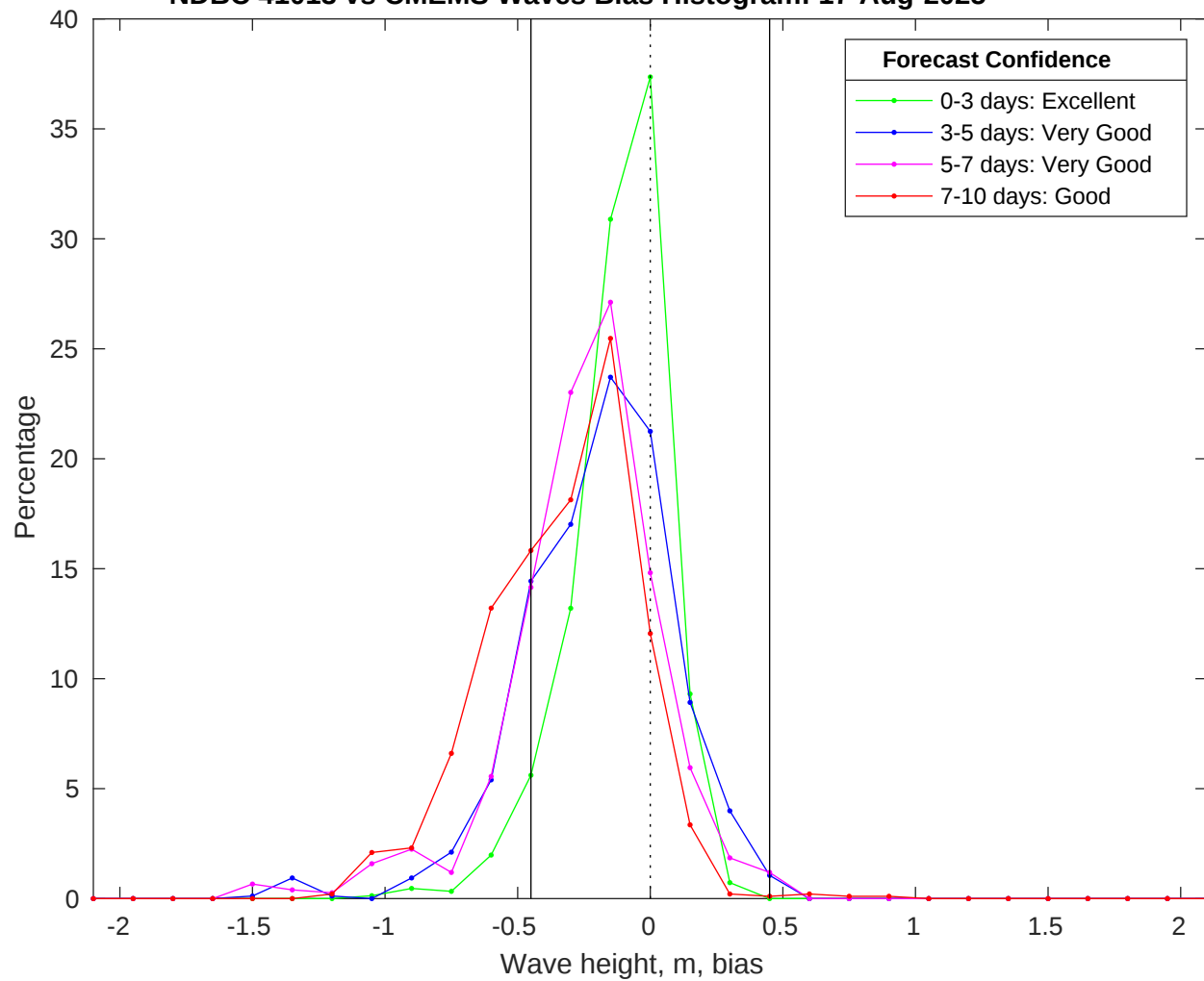
NDBC 41013 vs CMEMS Waves Bias Histogram: 17-Aug-2025
