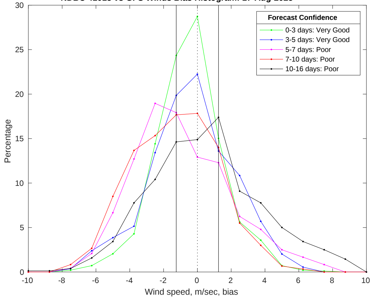
NDBC 41013 vs GFS Winds Bias Histogram: 17-Aug-2025
