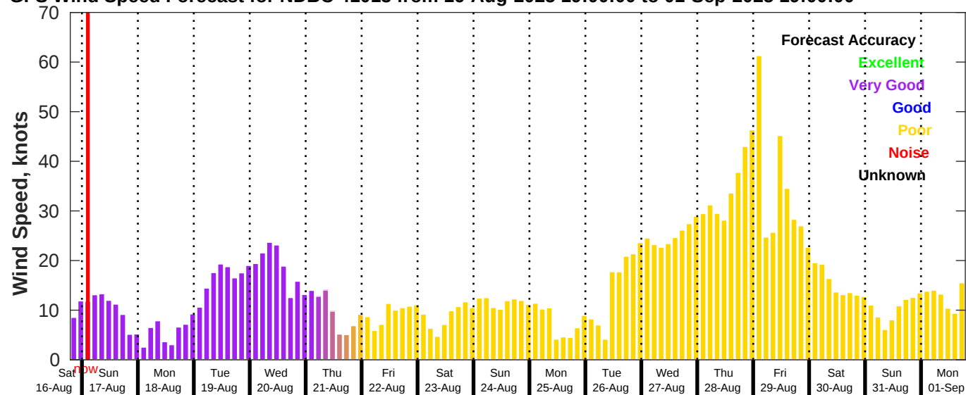
GFS Wind Speed Forecast for NDBC 41013 from 16-Aug-2025 19:00:00 to 01-Sep-2025 19:00:00
