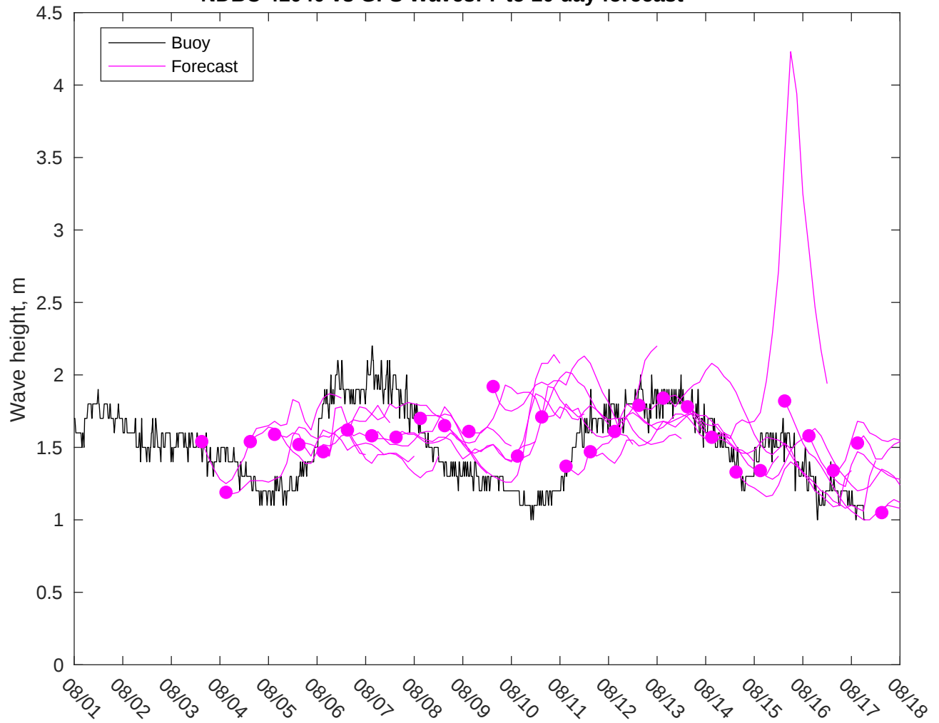
NDBC 41040 vs GFS Waves: 7 to 10 day forecast
