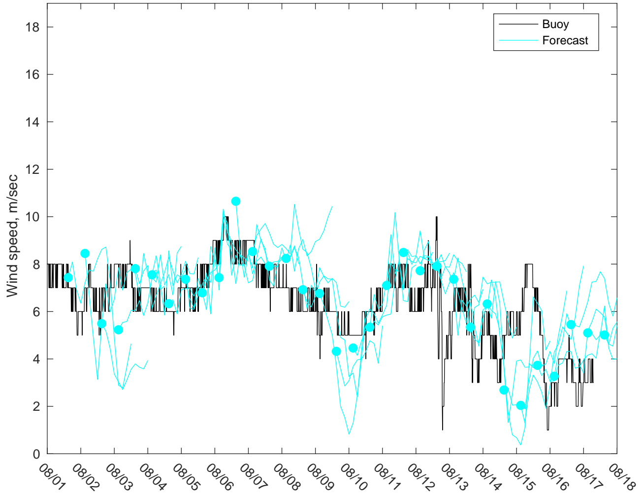
NDBC 41040 vs GFS Winds: 5 to 7 day forecast
