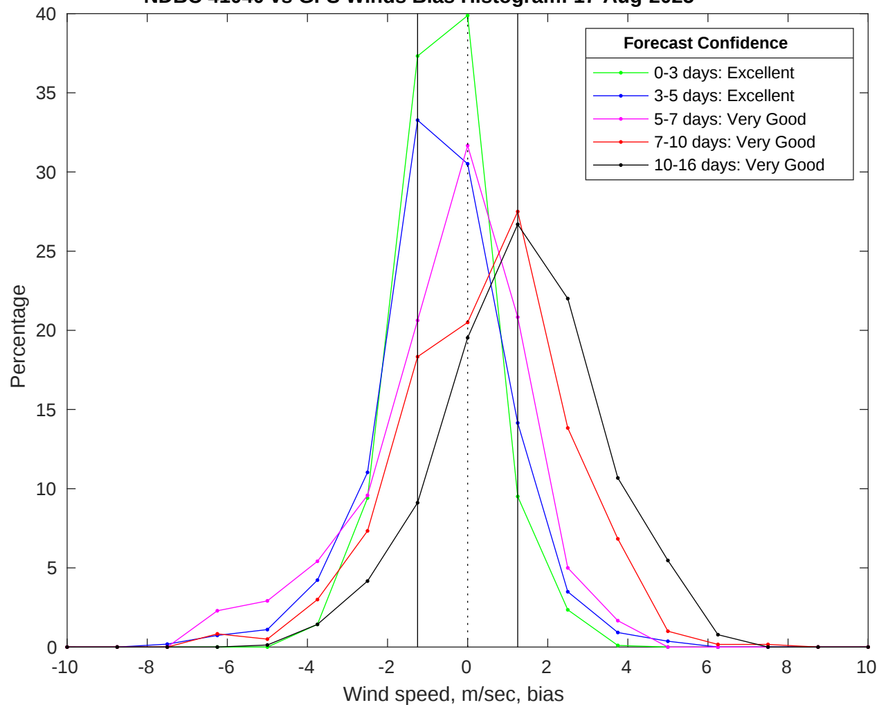
NDBC 41040 vs GFS Winds Bias Histogram: 17-Aug-2025
