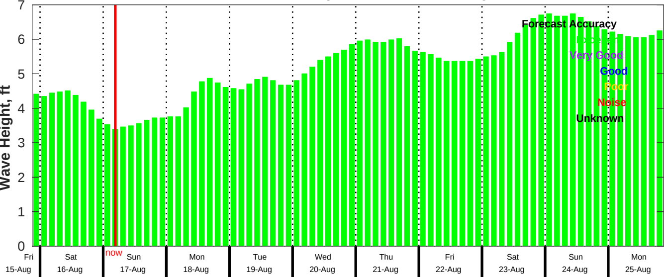
CMEMS Wave Forecast for NDBC 41040 from 15-Aug-2025 21:00:00 to 25-Aug-2025 21:00:00
