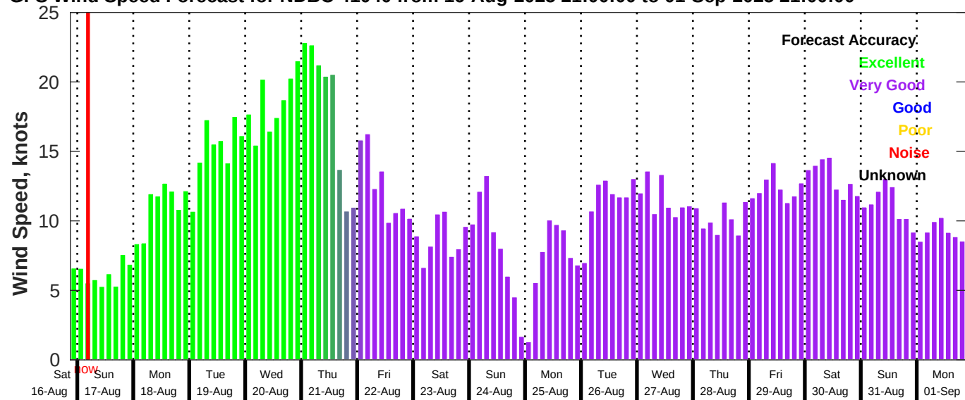
GFS Wind Speed Forecast for NDBC 41040 from 16-Aug-2025 21:00:00 to 01-Sep-2025 21:00:00
