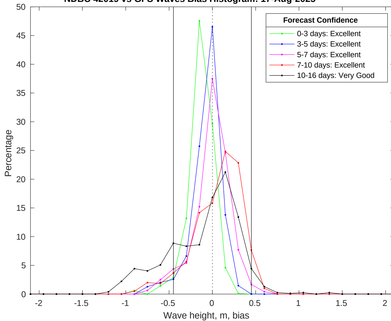
NDBC 42019 vs GFS Waves Bias Histogram: 17-Aug-2025
