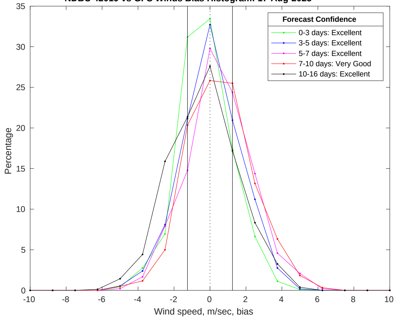
NDBC 42019 vs GFS Winds Bias Histogram: 17-Aug-2025
