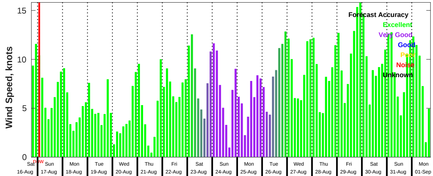
GFS Wind Speed Forecast for NDBC 42019 from 16-Aug-2025 18:00:00 to 01-Sep-2025 18:00:00
