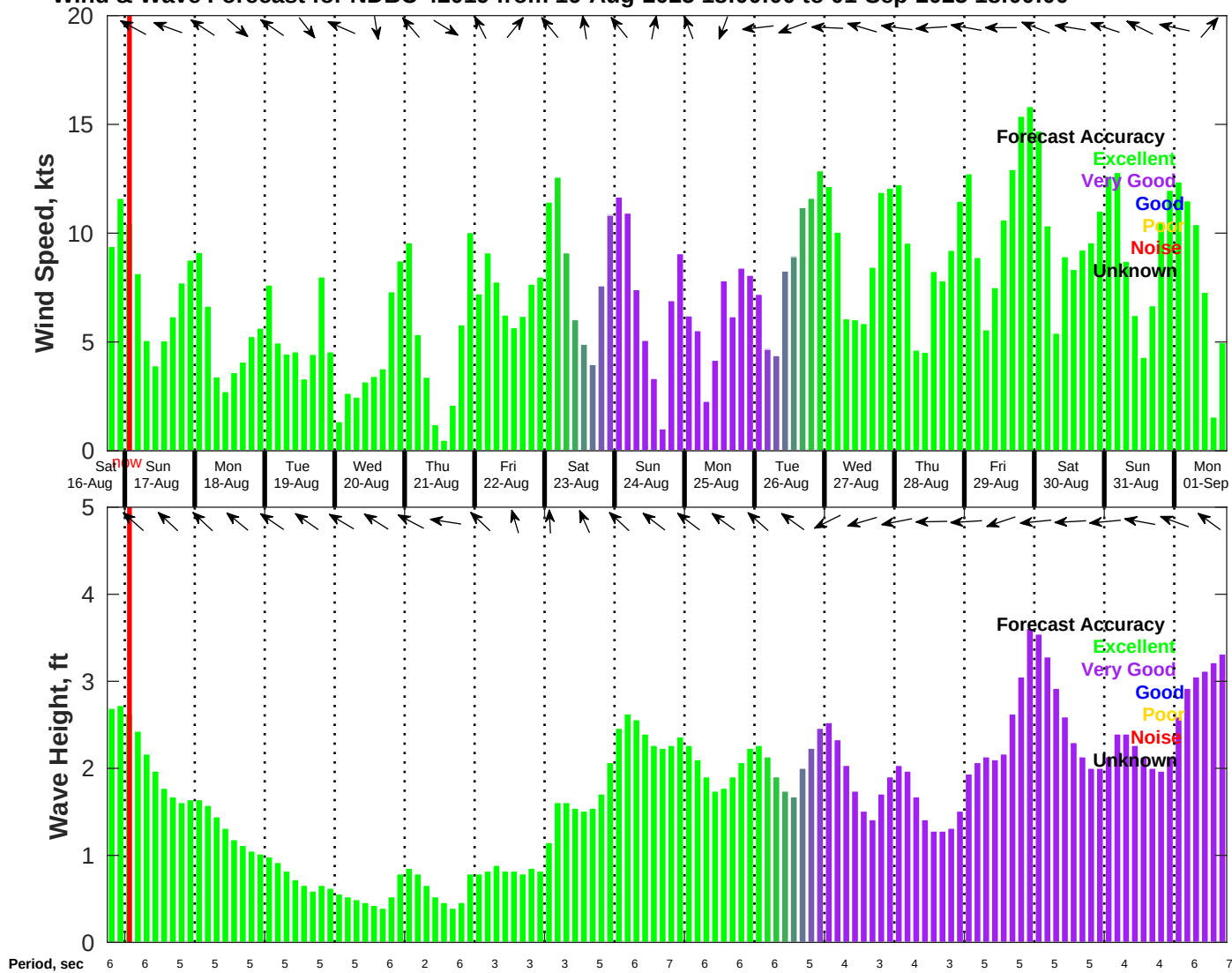
Wind & Wave Forecast for NDBC 42019 from 16-Aug-2025 18:00:00 to 01-Sep-2025 18:00:00
