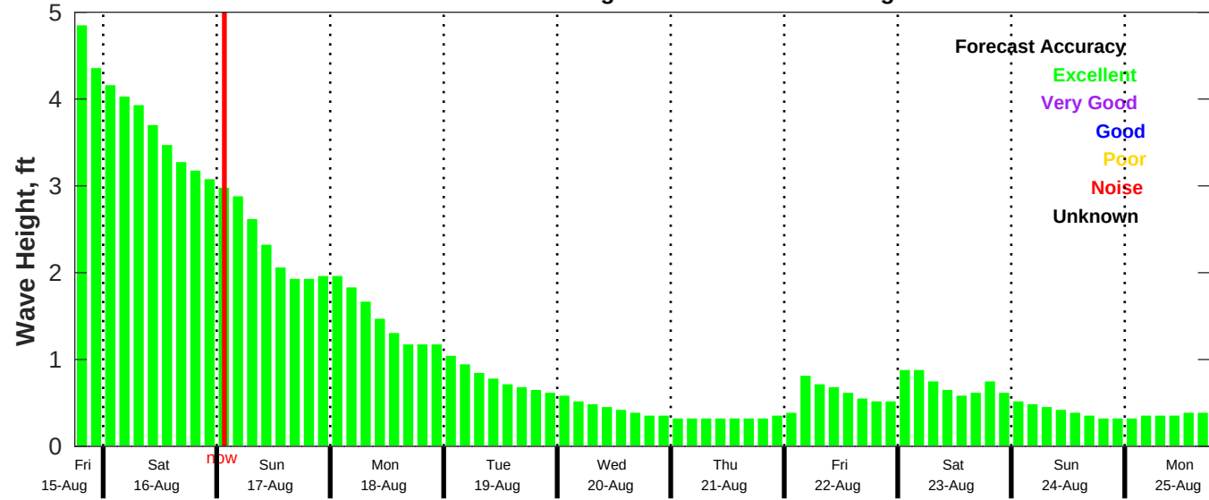
CMEMS Wave Forecast for NDBC 42020 from 15-Aug-2025 18:00:00 to 25-Aug-2025 18:00:00
