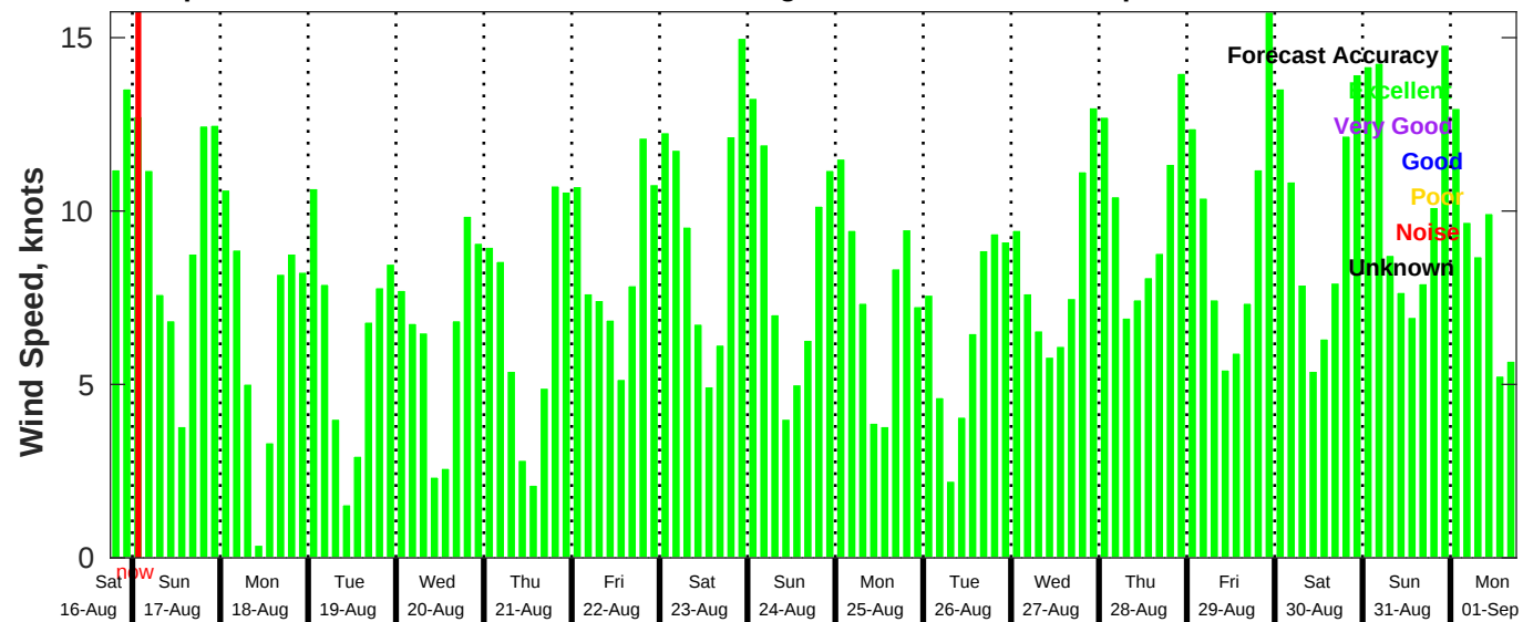
GFS Wind Speed Forecast for NDBC 42020 from 16-Aug-2025 18:00:00 to 01-Sep-2025 18:00:00
