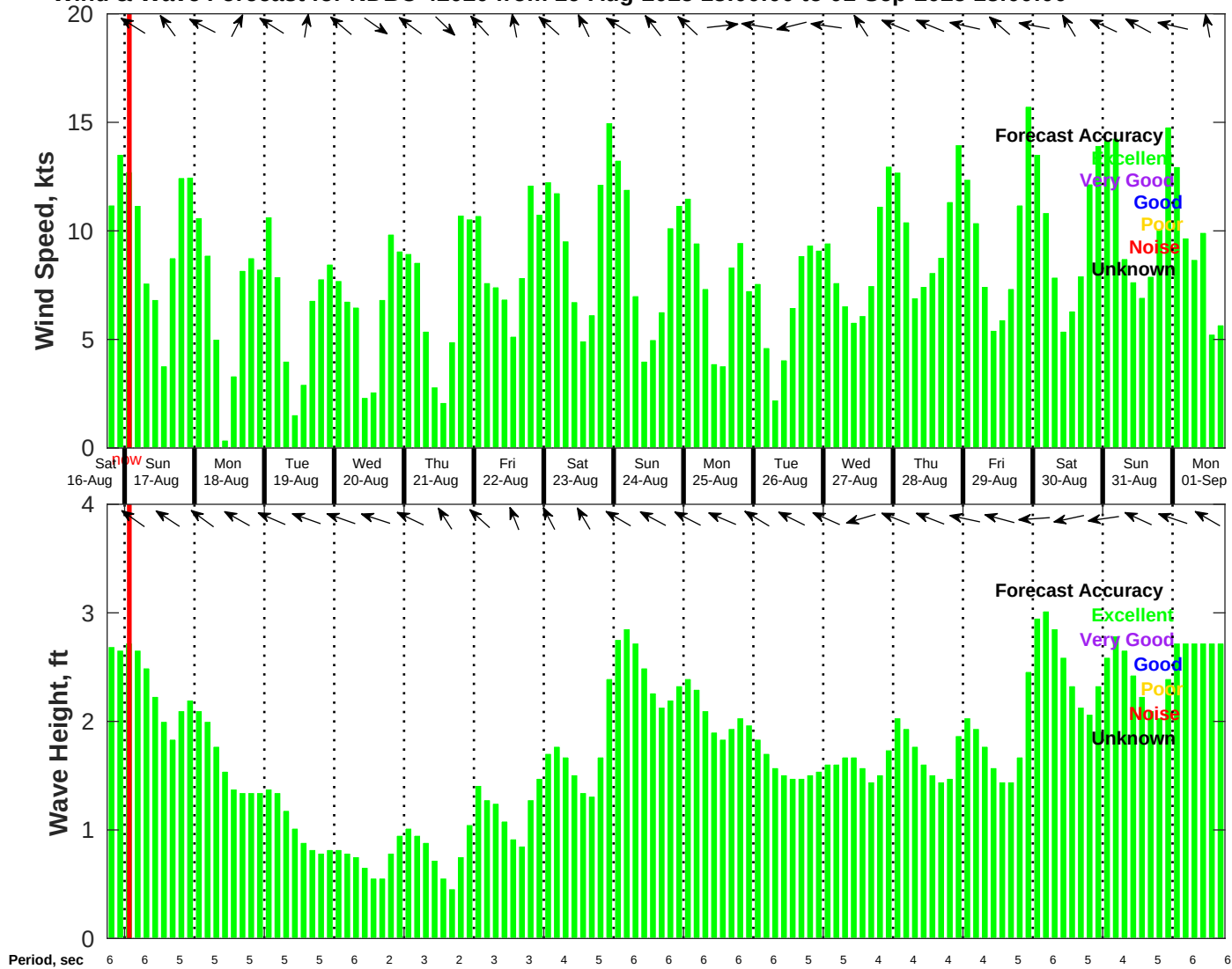
Wind & Wave Forecast for NDBC 42020 from 16-Aug-2025 18:00:00 to 01-Sep-2025 18:00:00
