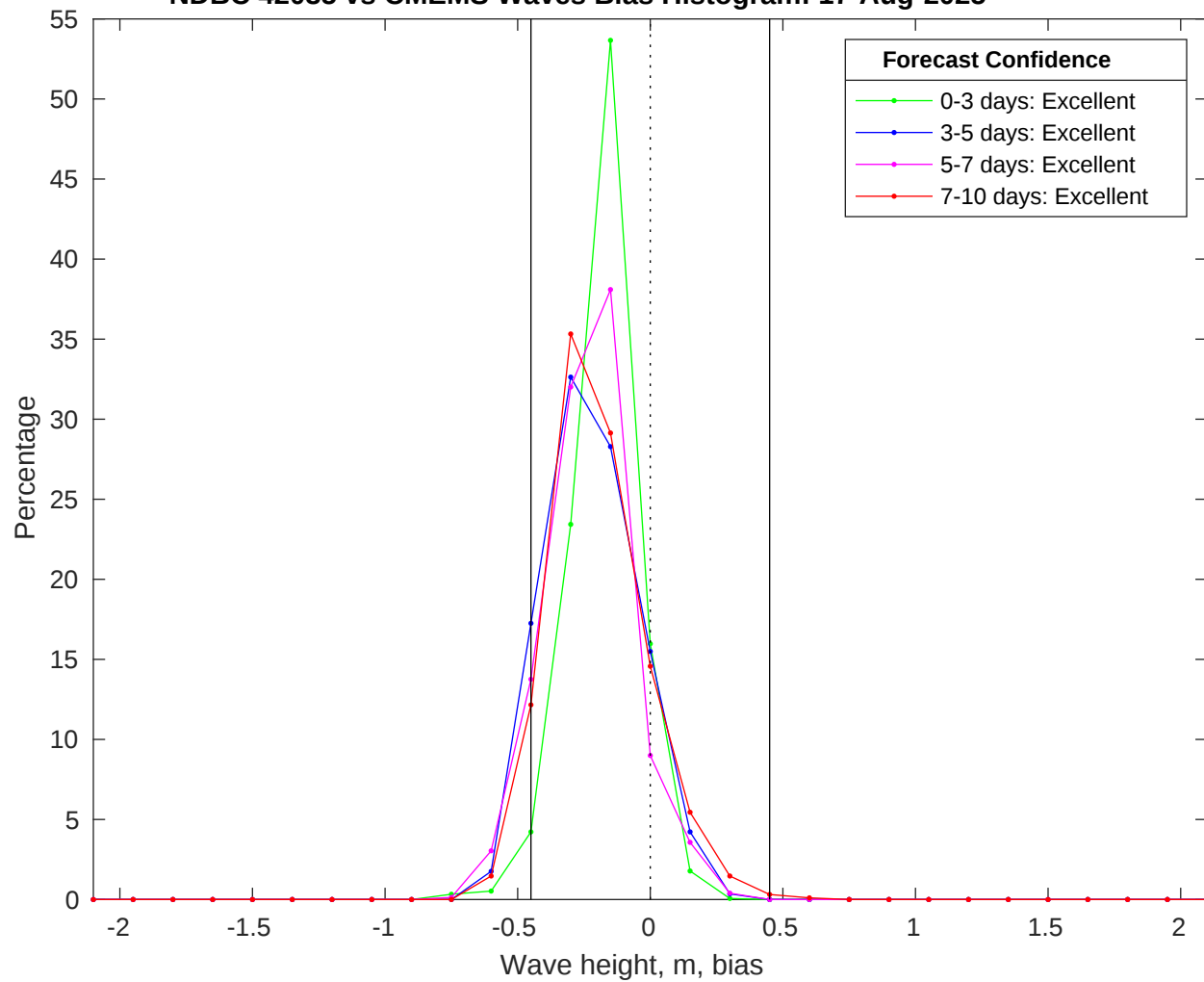
NDBC 42035 vs CMEMS Waves Bias Histogram: 17-Aug-2025
