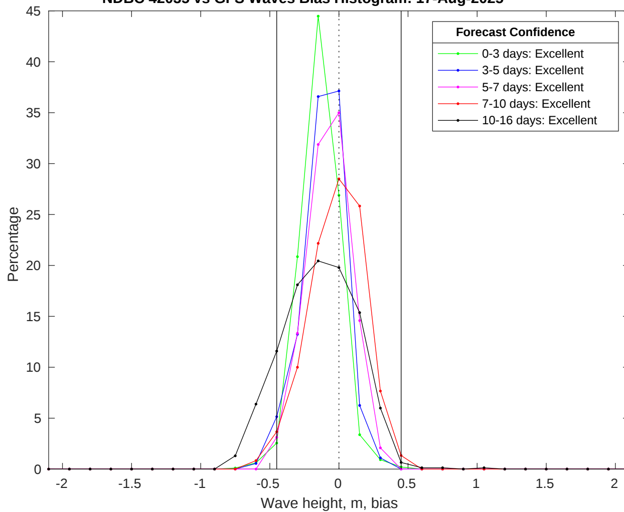
NDBC 42035 vs GFS Waves Bias Histogram: 17-Aug-2025
