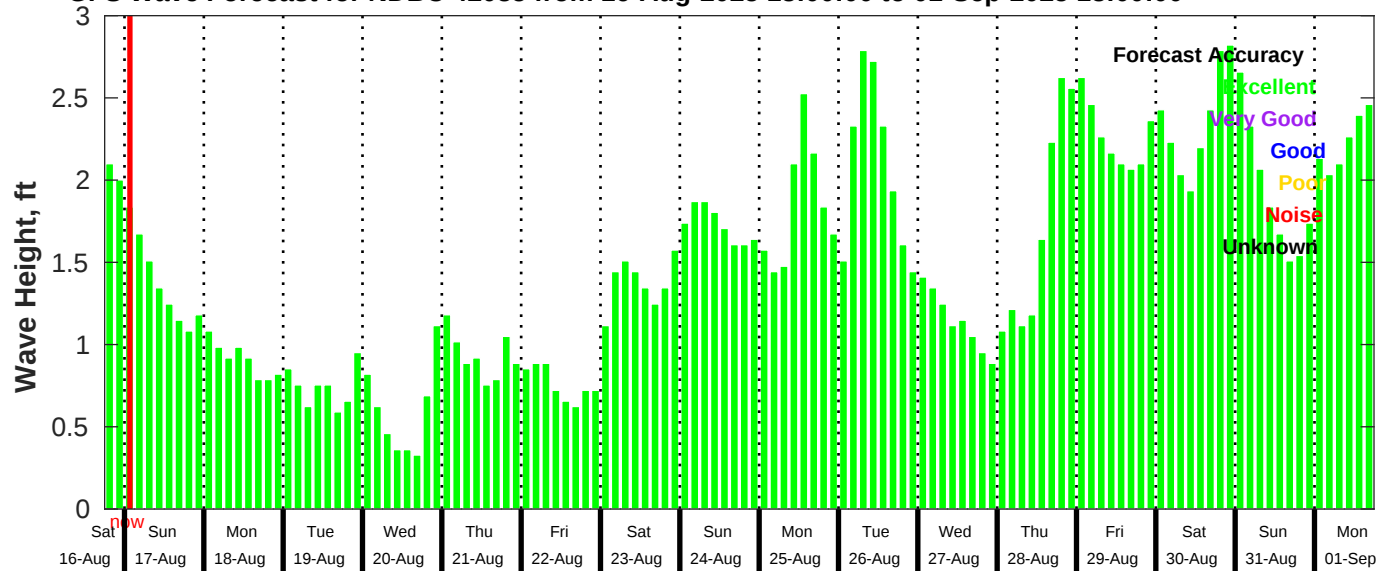
GFS Wave Forecast for NDBC 42035 from 16-Aug-2025 18:00:00 to 01-Sep-2025 18:00:00
