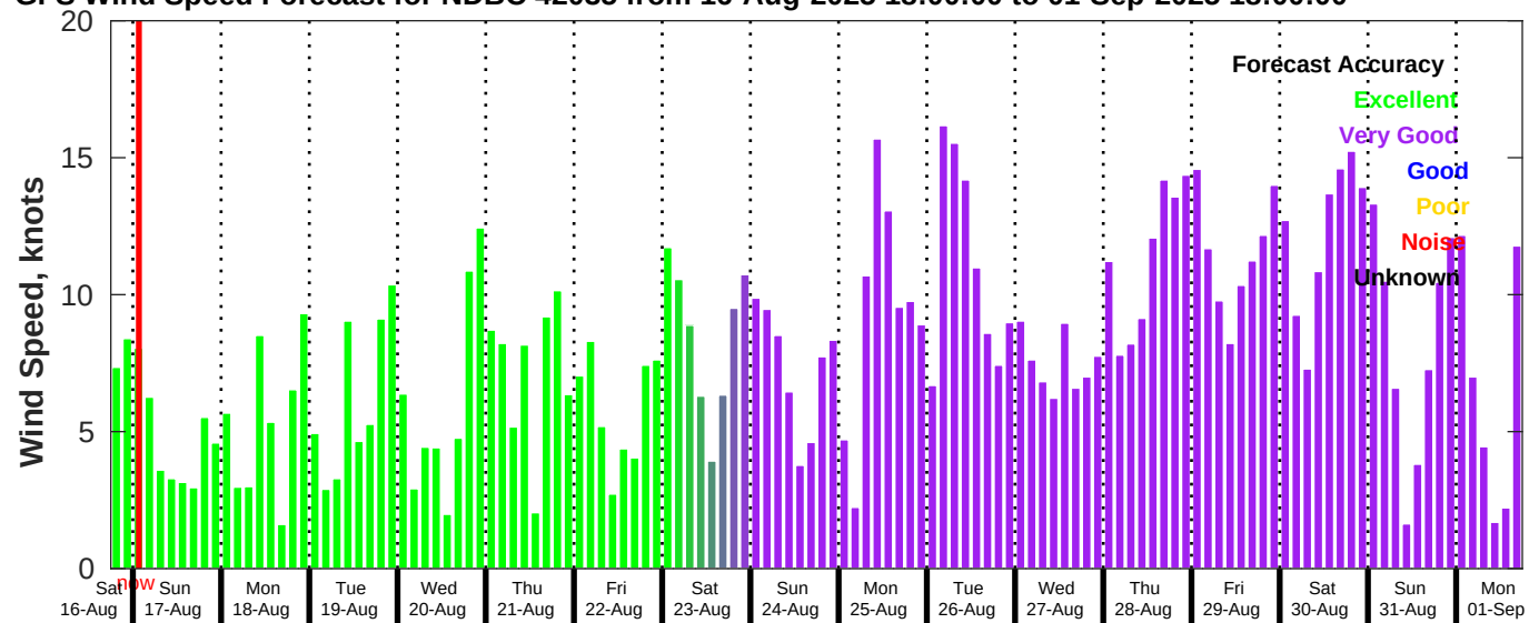
GFS Wind Speed Forecast for NDBC 42035 from 16-Aug-2025 18:00:00 to 01-Sep-2025 18:00:00
