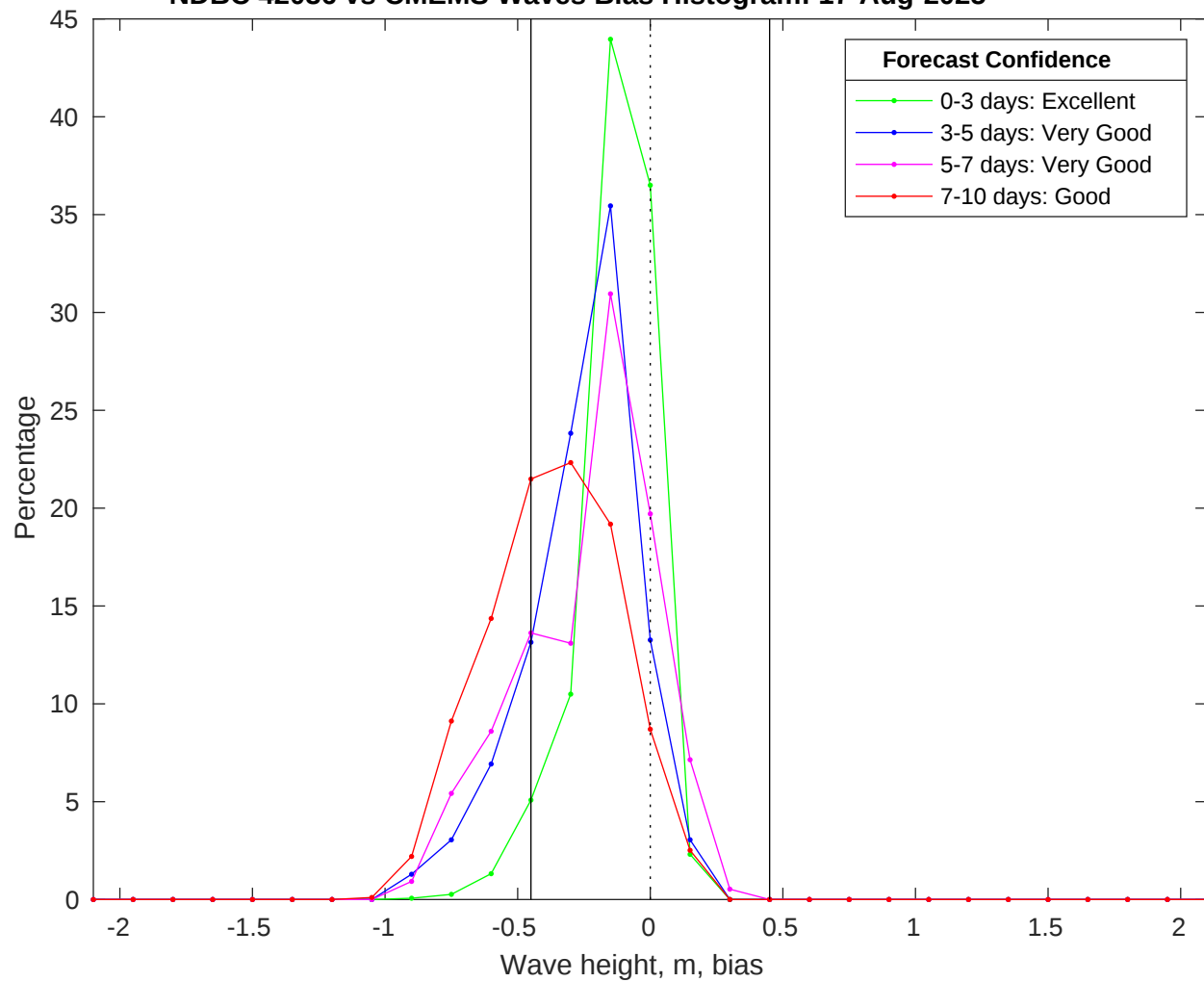
NDBC 42036 vs CMEMS Waves Bias Histogram: 17-Aug-2025
