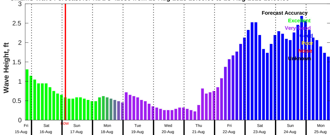
CMEMS Wave Forecast for NDBC 42036 from 15-Aug-2025 19:00:00 to 25-Aug-2025 19:00:00
