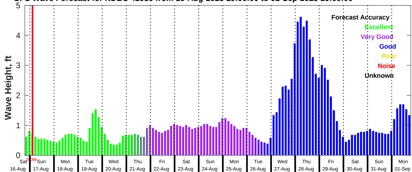
GFS Wave Forecast for NDBC 42036 from 16-Aug-2025 19:00:00 to 01-Sep-2025 19:00:00
