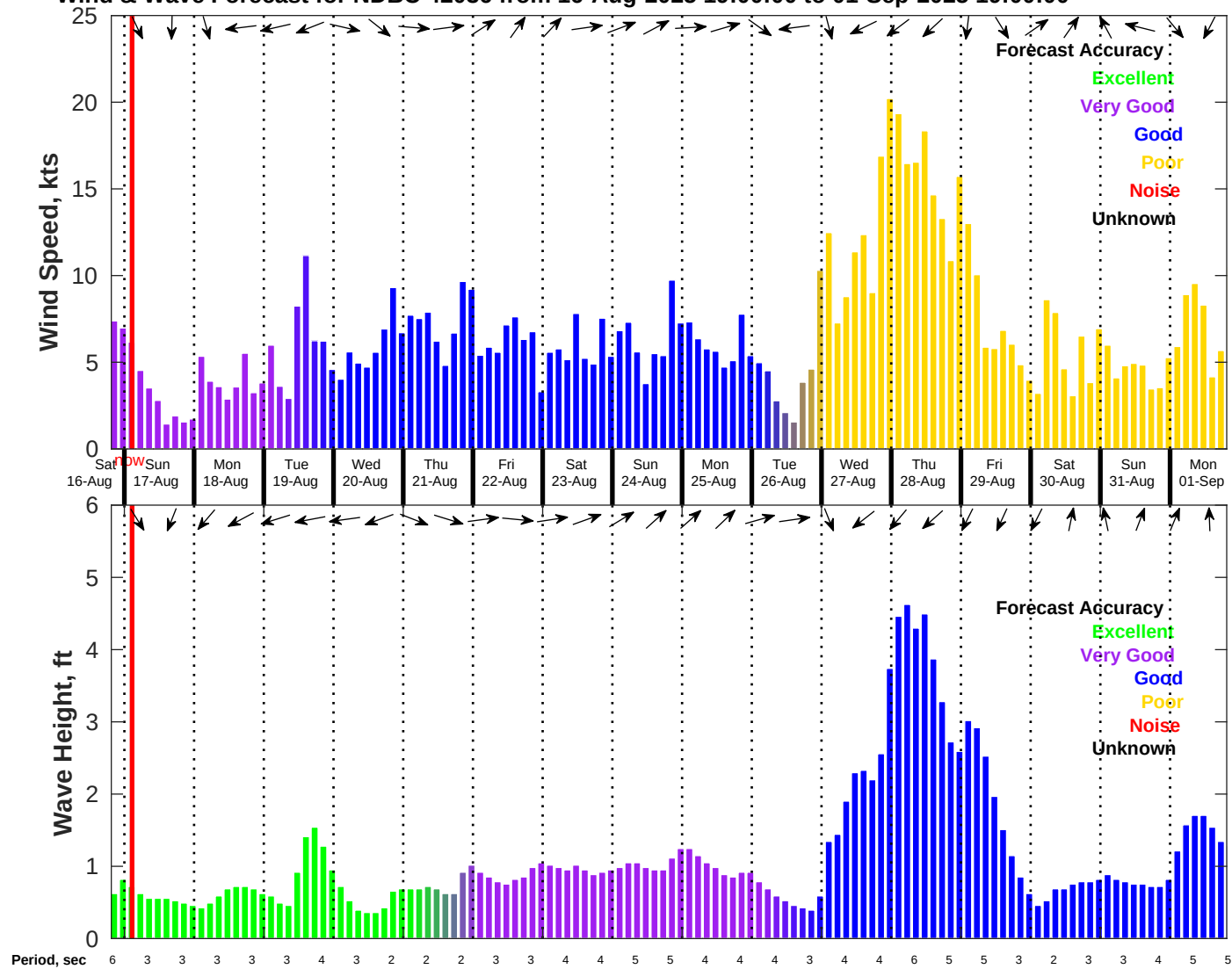
Wind & Wave Forecast for NDBC 42036 from 16-Aug-2025 19:00:00 to 01-Sep-2025 19:00:00
