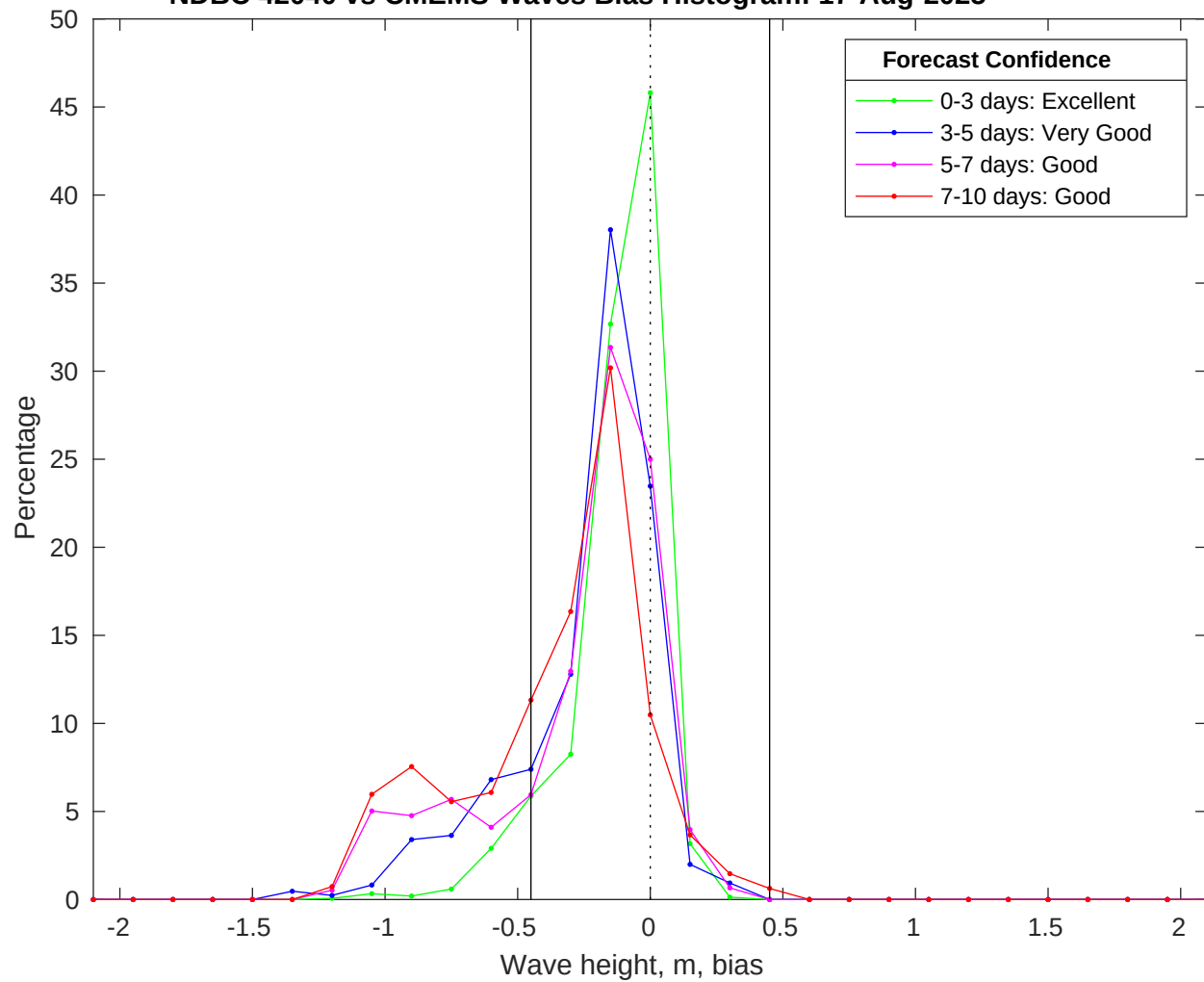
NDBC 42040 vs CMEMS Waves Bias Histogram: 17-Aug-2025
