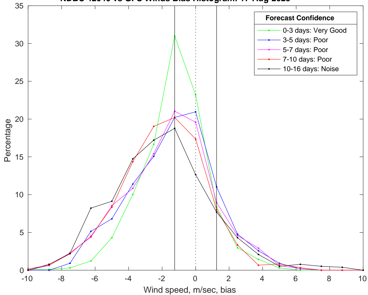
NDBC 42040 vs GFS Winds Bias Histogram: 17-Aug-2025
