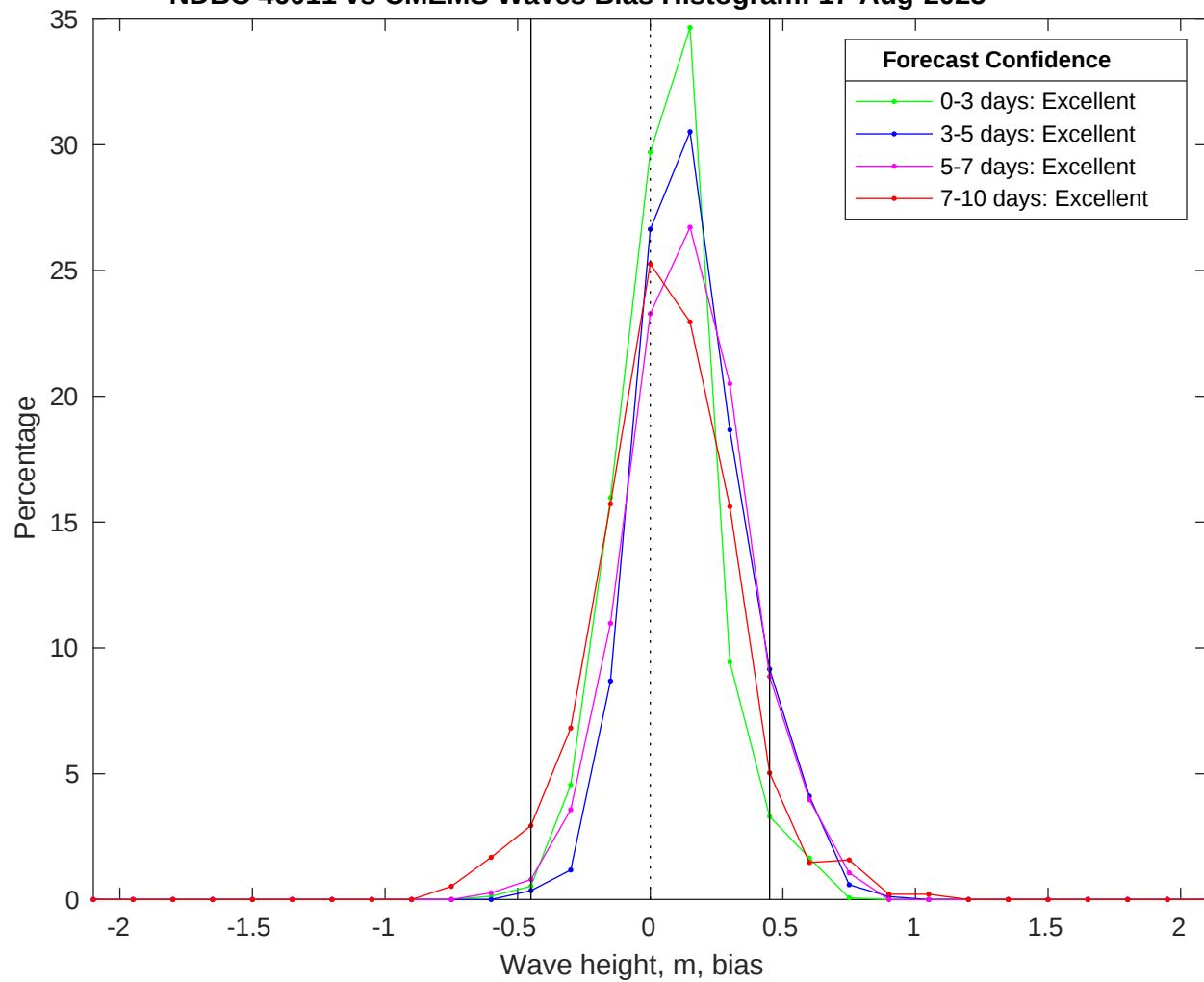
NDBC 46011 vs CMEMS Waves Bias Histogram: 17-Aug-2025
