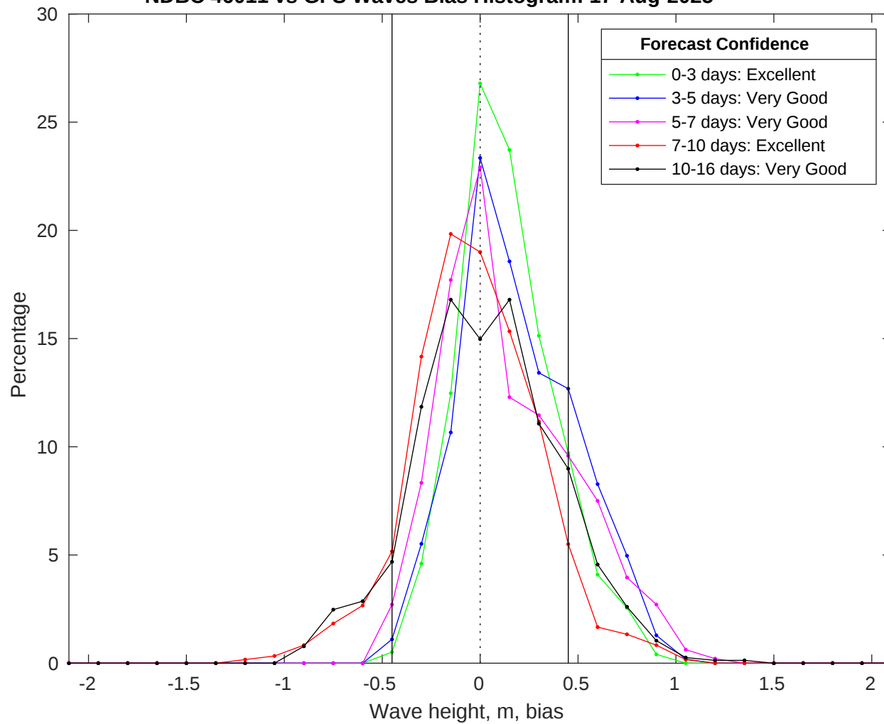
NDBC 46011 vs GFS Waves Bias Histogram: 17-Aug-2025
