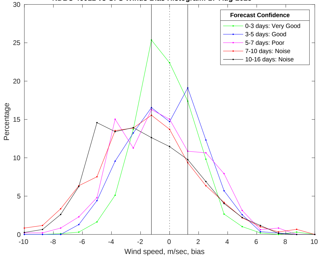
NDBC 46011 vs GFS Winds Bias Histogram: 17-Aug-2025
