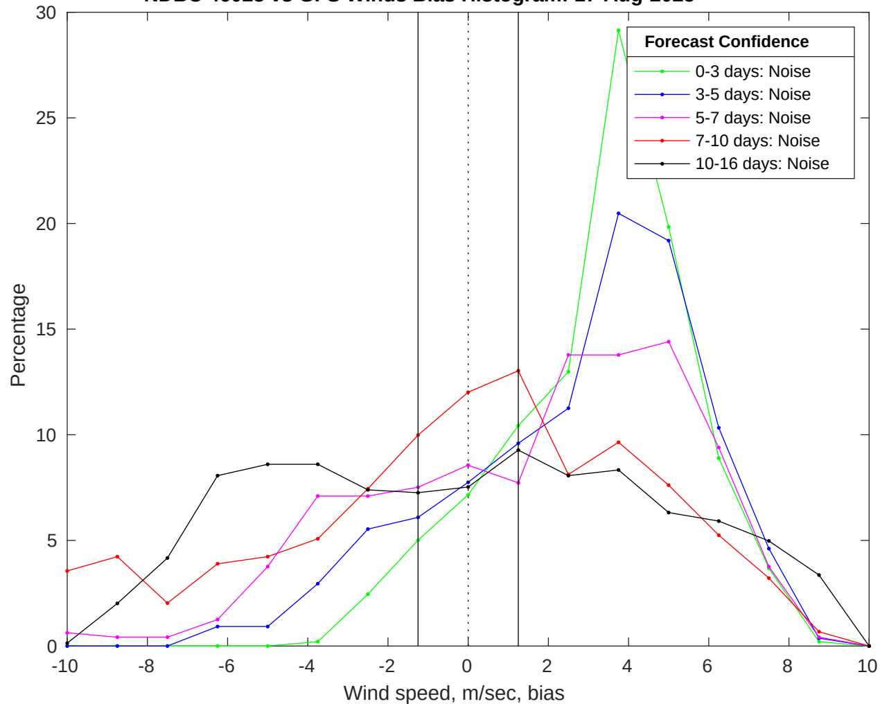
NDBC 46028 vs GFS Winds Bias Histogram: 17-Aug-2025
